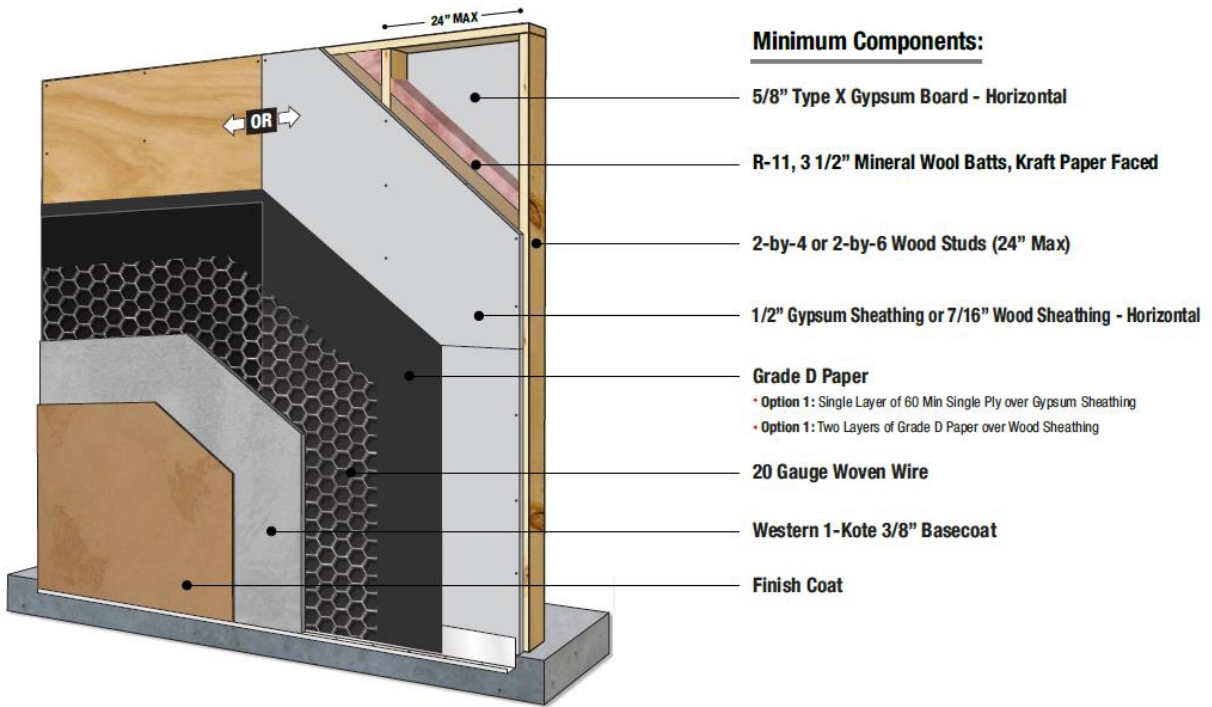
Figure 9 - One Hour Firewall Assembly No. 3 (Table 3)
