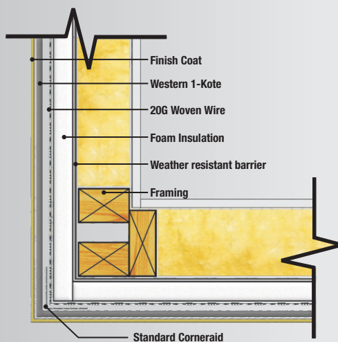
Corner Square Termination
