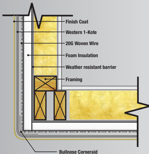
Corner Bullnose Termination
