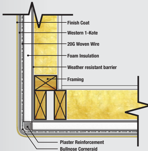
Corner with Reinforcement
